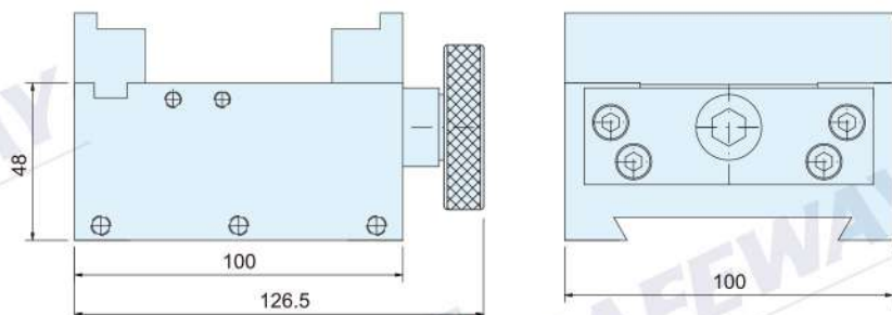
虎鉗滑座 YES VISE ORDER NO.42100006 MODEL: MV-100100PS
