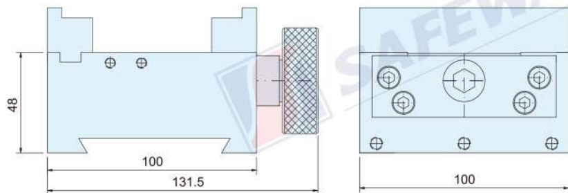
虎鉗滑座 YES VISE ORDER NO.42100004 MODEL: MV-100100CS
